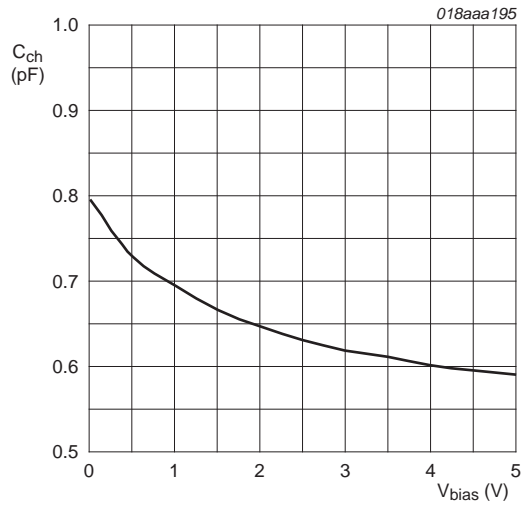
Fig 3. Channel capacitance as a function of bias voltage; typical values
