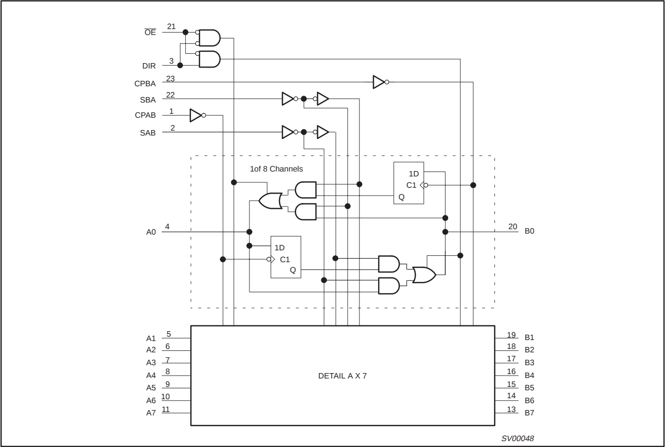
LOGIC DIAGRAM
