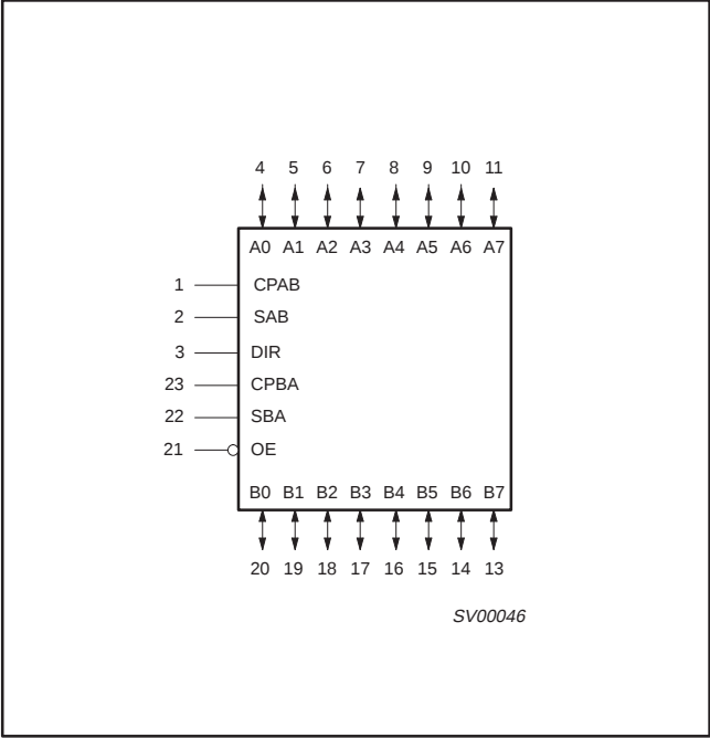
LOGIC SYMBOL
