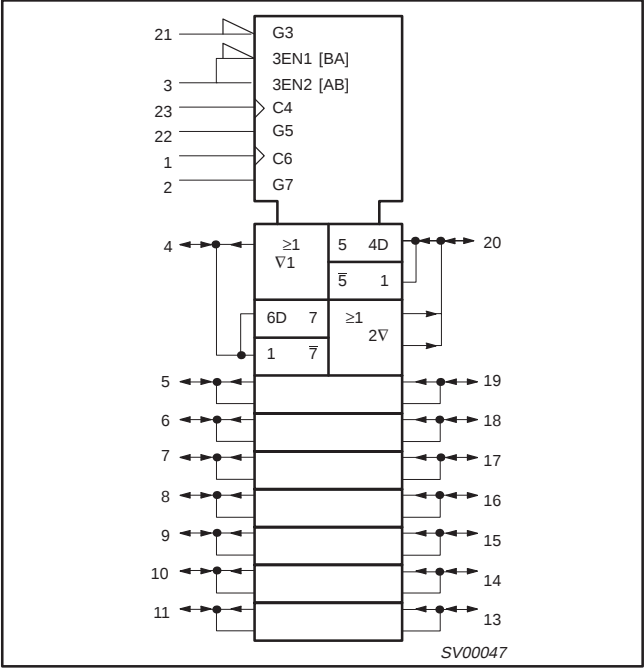
LOGIC SYMBOL (IEEE/IEC)
