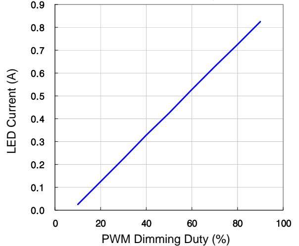
LED Current vs PWM Dimming Duty ( C_4 open, PWM Frequency=500Hz)
