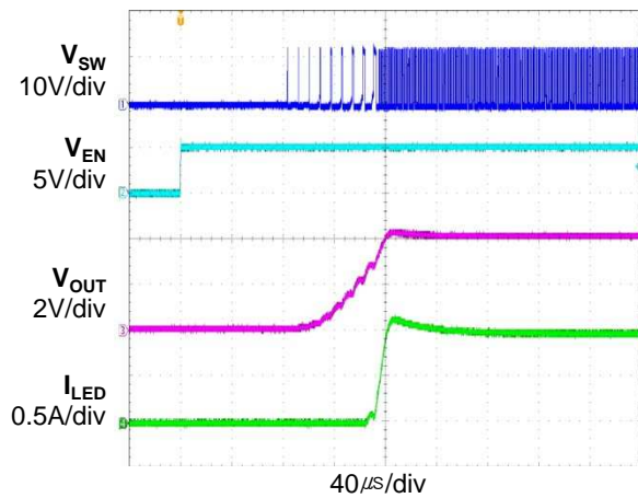
Enable Start-up ( C_4 open)
