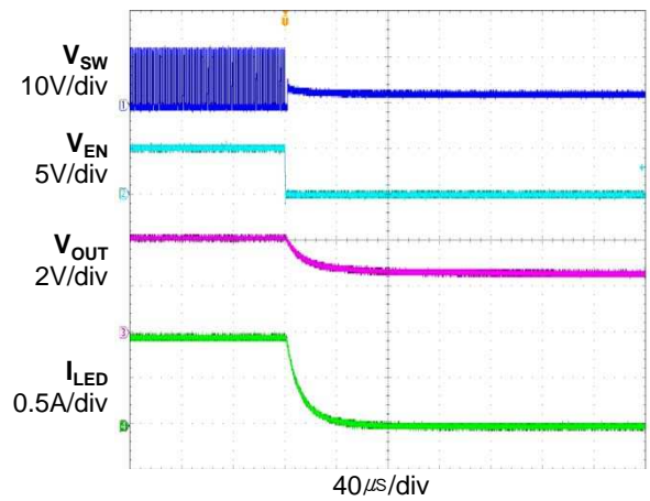
Enable Turn-off ( C_4 open)
