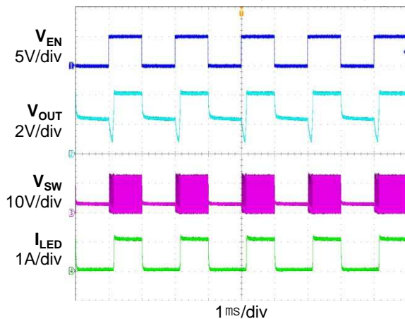
PWM Dimming Through Enable ( C_4 open, PWM Frequency=500Hz, Duty=50%)
