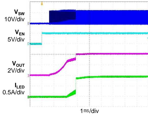
Enable Start-up ( C_4=100nF )
