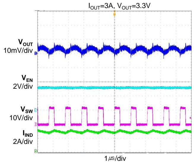
Steady State Operation
