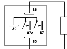
2A Wiring Diagram (Bottom View)
