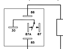
1C Wiring Diagram (Bottom View)
