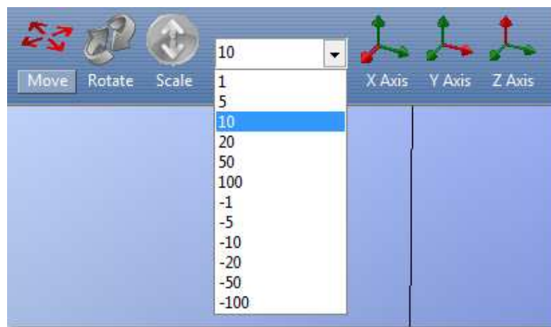
Windows version
