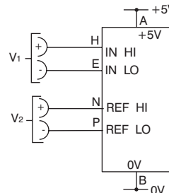
Measuring the ratio of two voltages Reading = 1000 V_1/V_2 50mV < V_2 < 200mV V_1 < 2V_2
