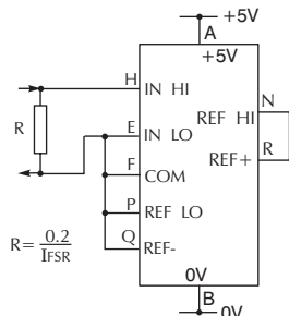
Measuring Current.
