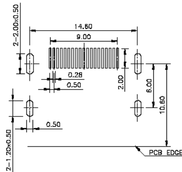
PCB RECOMMENDED LAYOUT (TOP VIEW) Tolerance \pm 0.05
