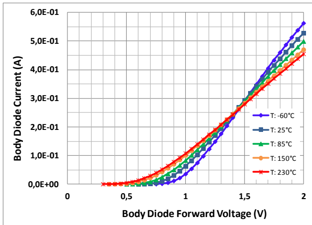
Figure 7. Body Diode Forward Current ( I_{FD} ) vs Forward Voltage for several case temperature. V_{GS}=0V .
