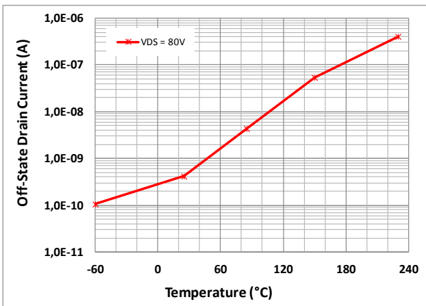
Figure 5. Off-State Drain Current ( I_{DSS} ) vs Case Temperature. V_{DS}=80V , V_{GS}=0V .
