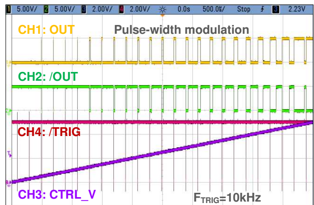
Figure 17. Waveforms in Pulse Width Modulation (PWM): externally retrigged monostable configuration with modulating signal on CONTROL_V (see Figure 23). V_{DD}=5.0V , F_{TRIG}=10kHz , R_A=R_B=15k , C=1.06nF .
