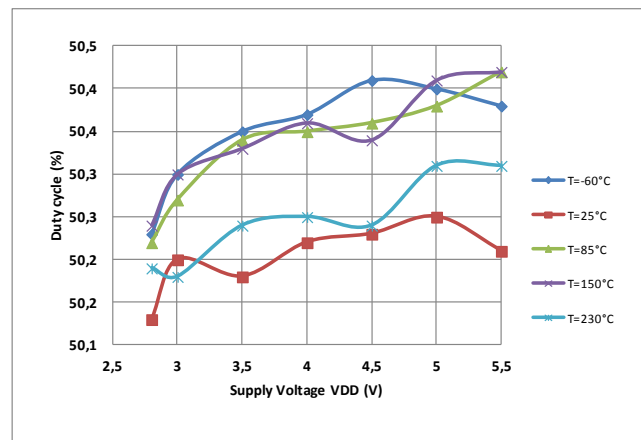
Figure 11. Duty-ratio in astable mode vs. Supply Voltage (see Figure 19). R_A=1k , R_B=1k , C=9.7nF .
