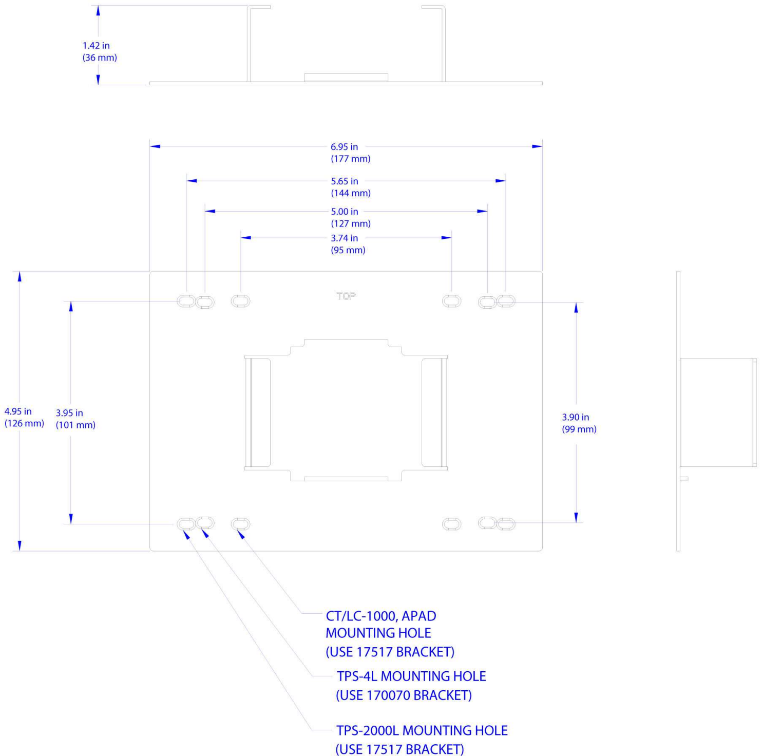
TSW-1050-RMB-3 – Dimensional Drawing
