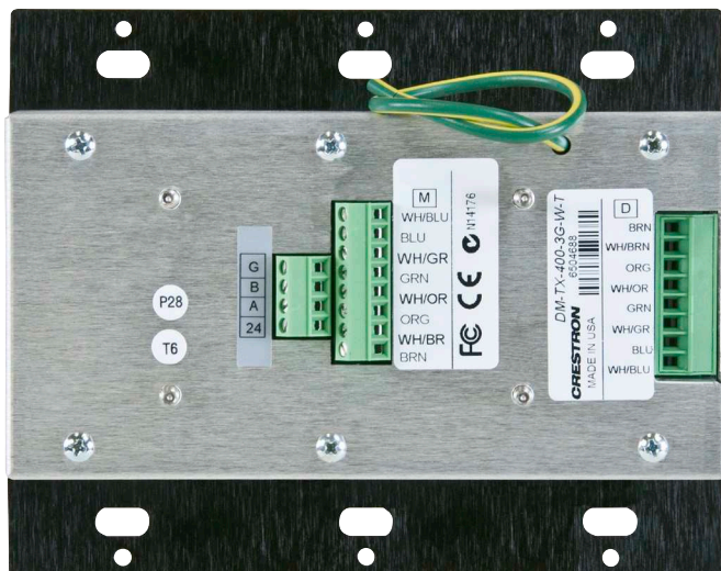
DM-TX-400-3G-W-T – Front and Rear Views
