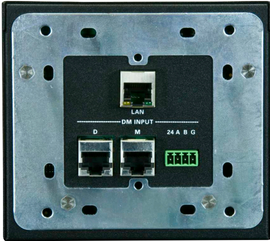
DM-RMC-100 – Rear View
