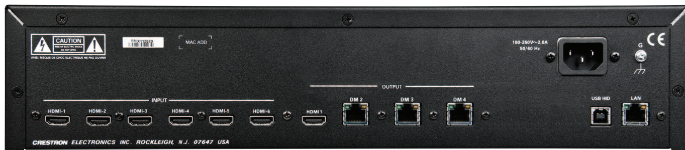
DM-MD6X4 – Rear View
