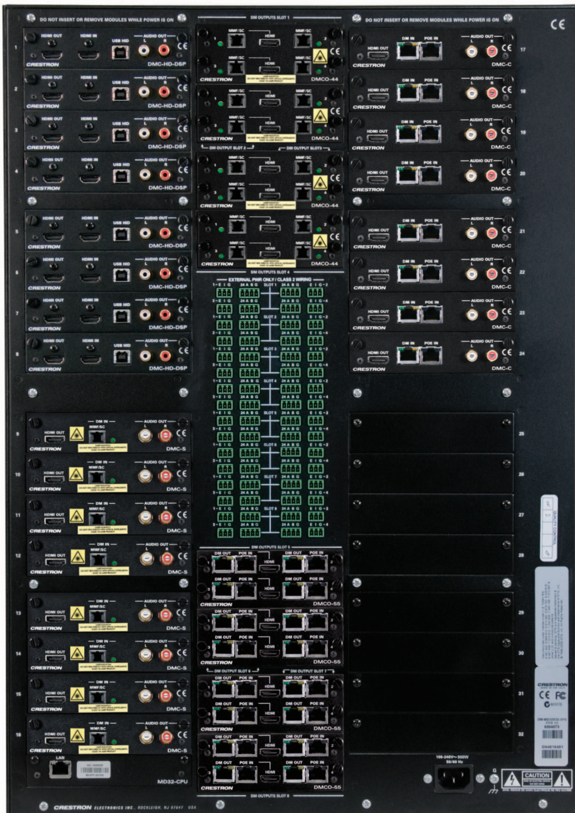
DM-MD32X32-RPS – Rear view with I/O cards installed
