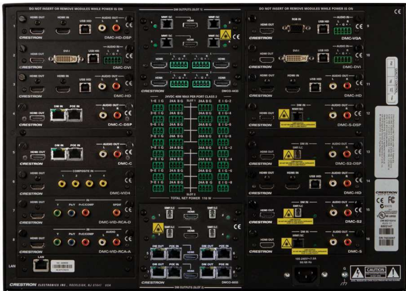
DM-MD16X16 – Rear view with I/O cards installed
