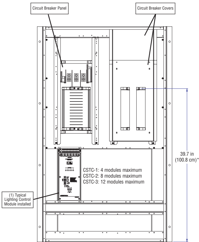
Front View – with front covers removed (CSTC-1-120-60 shown)
