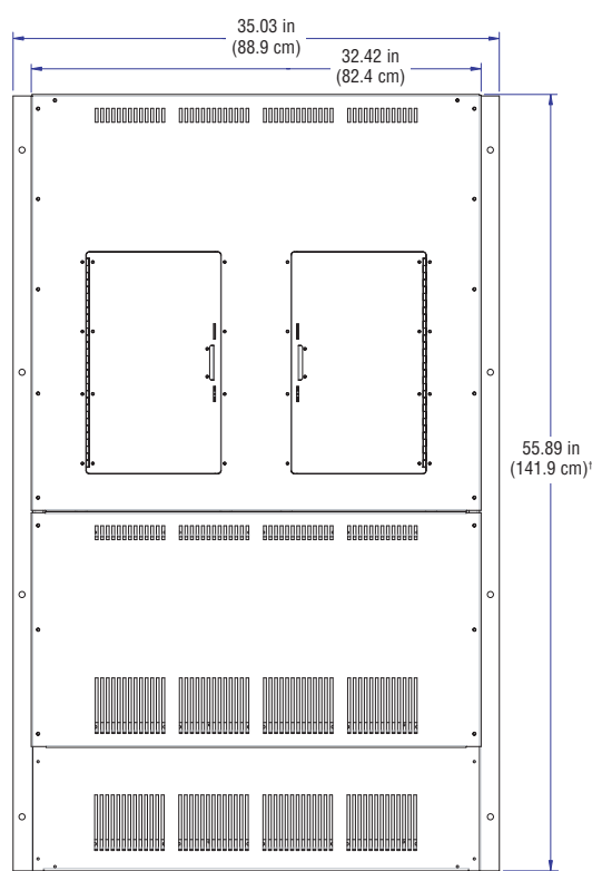
Front View – with front covers installed (CSTC-1-xxx-60 shown)
