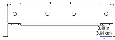
Bottom View – All Models
