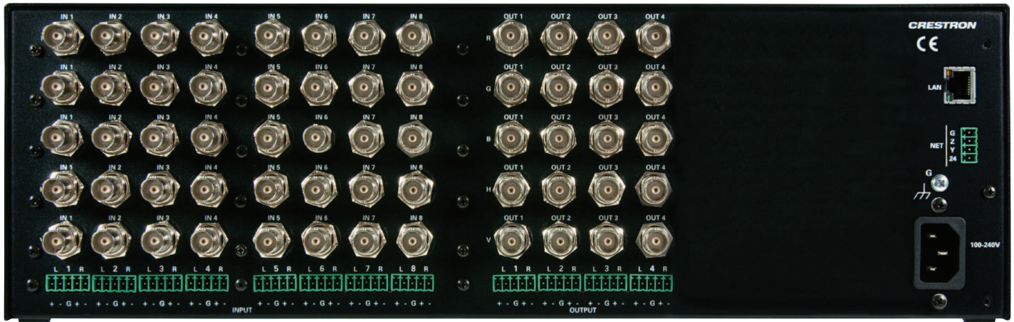
CEN-RGBHVHB8X4 – Rear View
