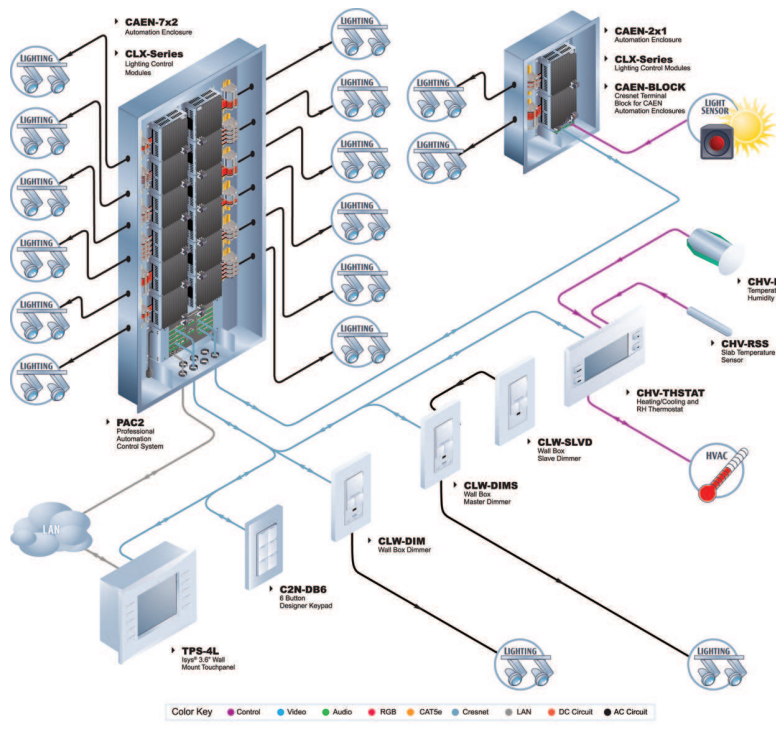
CLX and CLXI Series Lighting Control Modules
