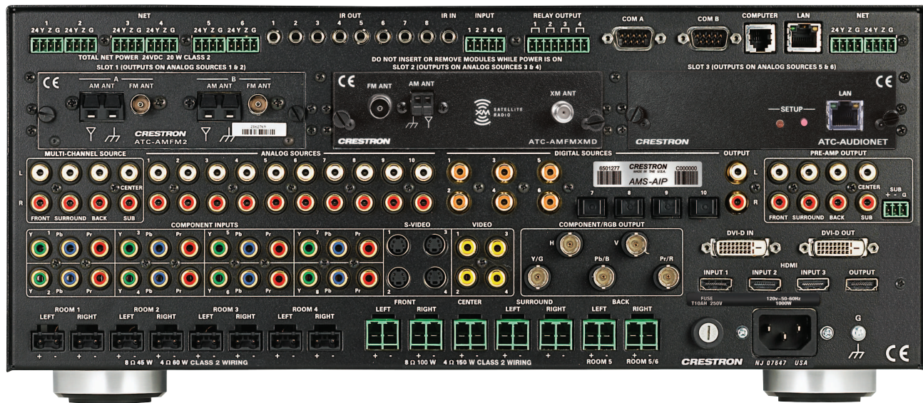
AMS-AIP – Rear View with ATC-AMFM2, ATC-AMFMXMD, and ATC-AUDIONET Tuner Cards
