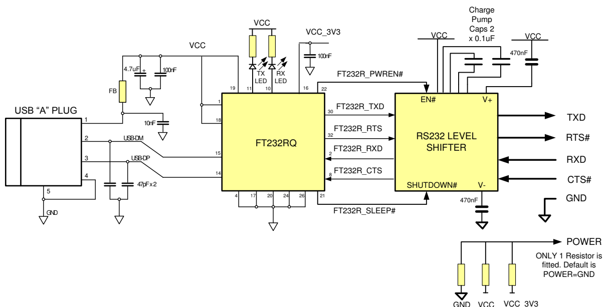
Figure 6.1 Circuit Schematic of PCB Used in the USB to RS232 Serial Converter Cable
