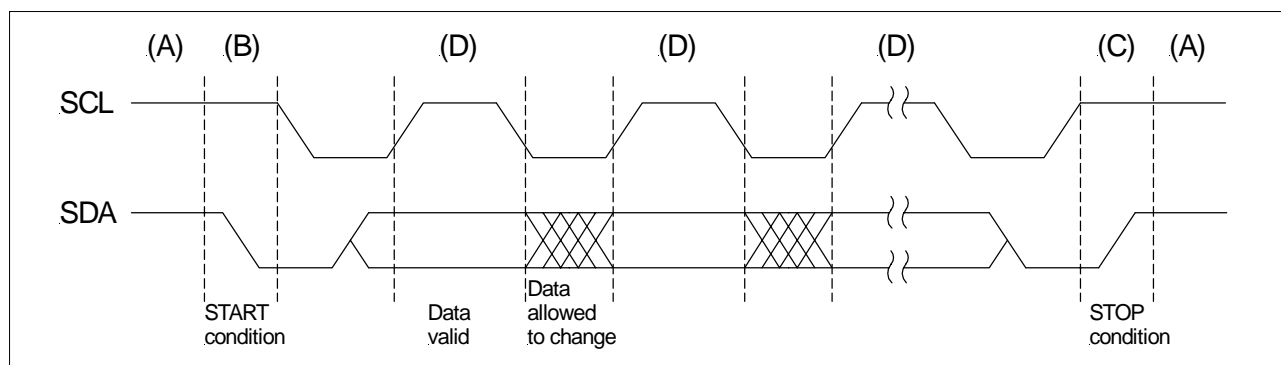
Fig. 1: I 2 C bus protocol
