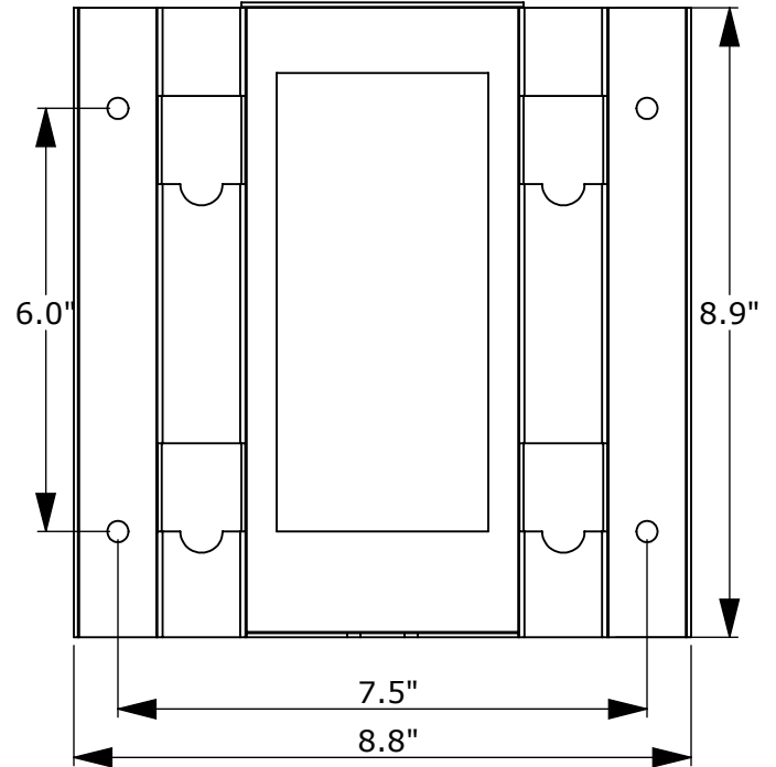
Wall Plate
