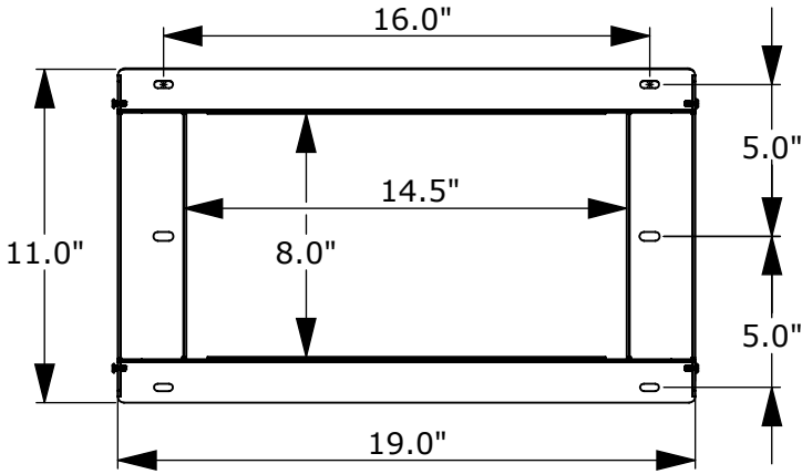
Wall Plate
