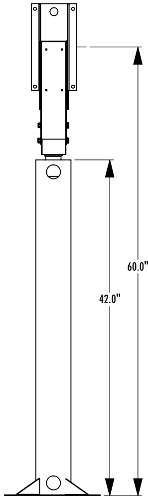
Front View
