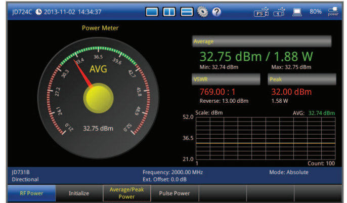
Power Meter
