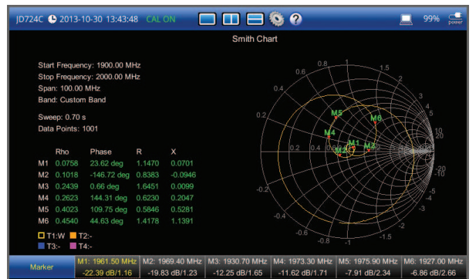
Smith Chart
