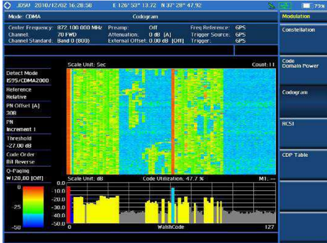
CDMA codogram
