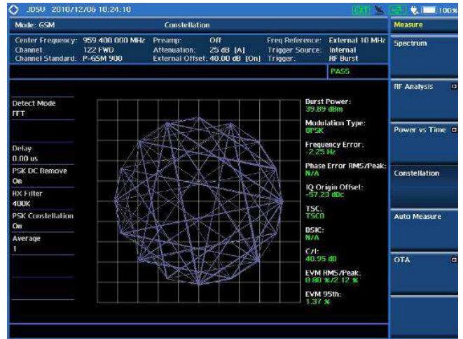
GSM constellation
