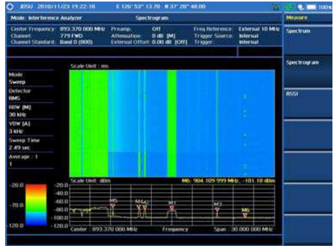
Spectrogram
