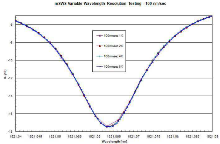
Figure 1. Example of ultra-high resolution where all data was collected at 100 nm/s sweep speed
