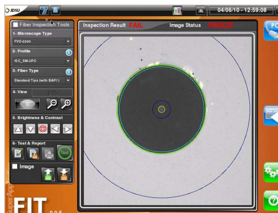
Figure 4. Connector Inspection interface
