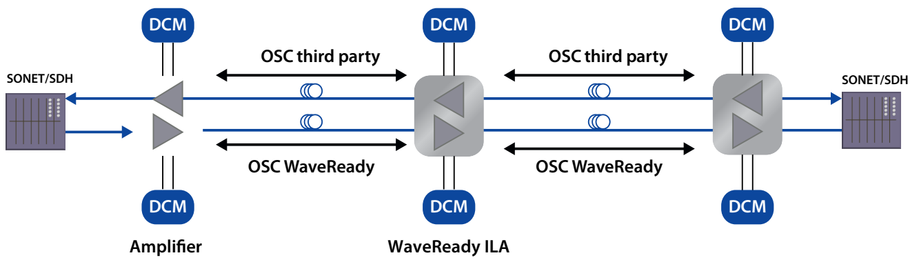
Figure 2. WaveReady ILA OSC and interop deployment
