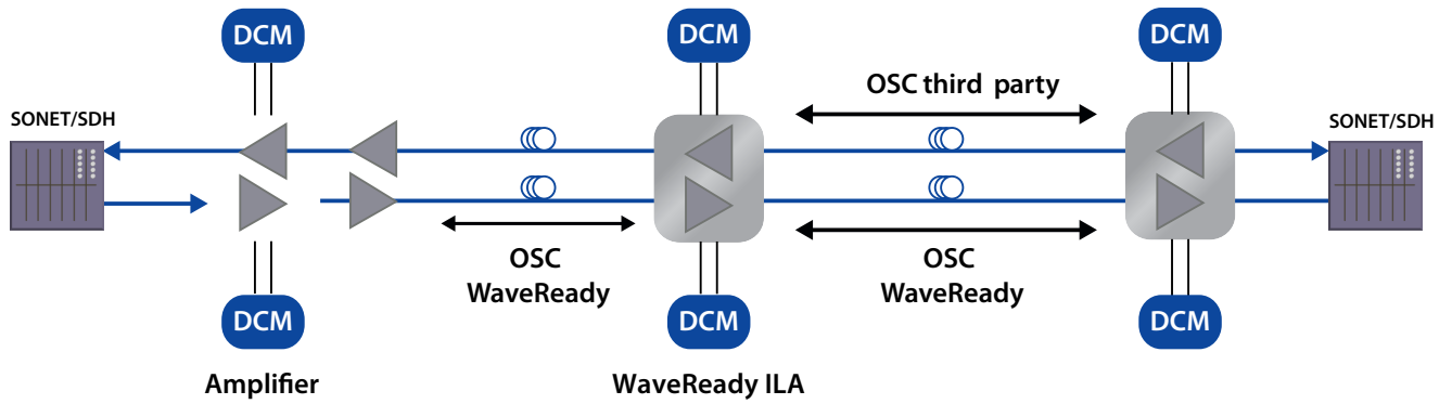
Figure 1. WaveReady ILA complexity reduction
