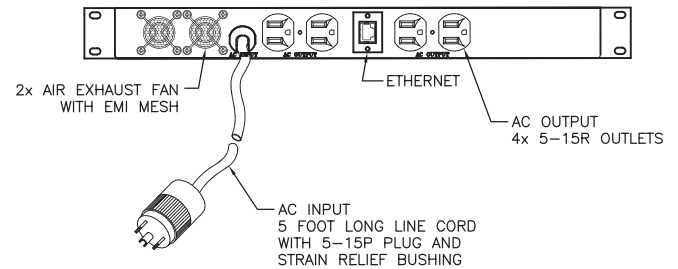
REAR VIEW
