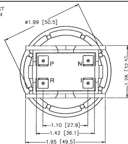
C1161AB Counter
