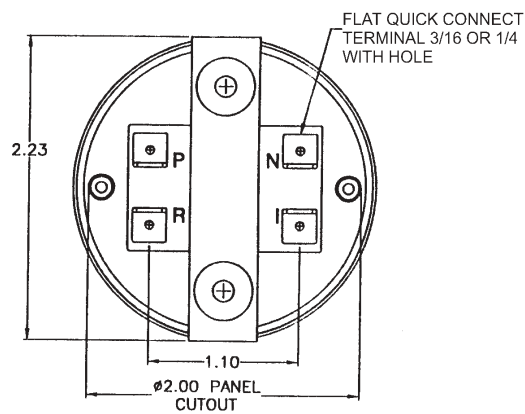
C1151AB Counter
