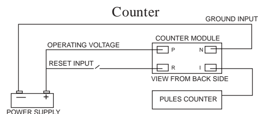
C1161AB Counter
