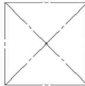
Recommended Panel Cut-out 68 x 68mm (2.68in) +0.7(0.03in) -0mm
