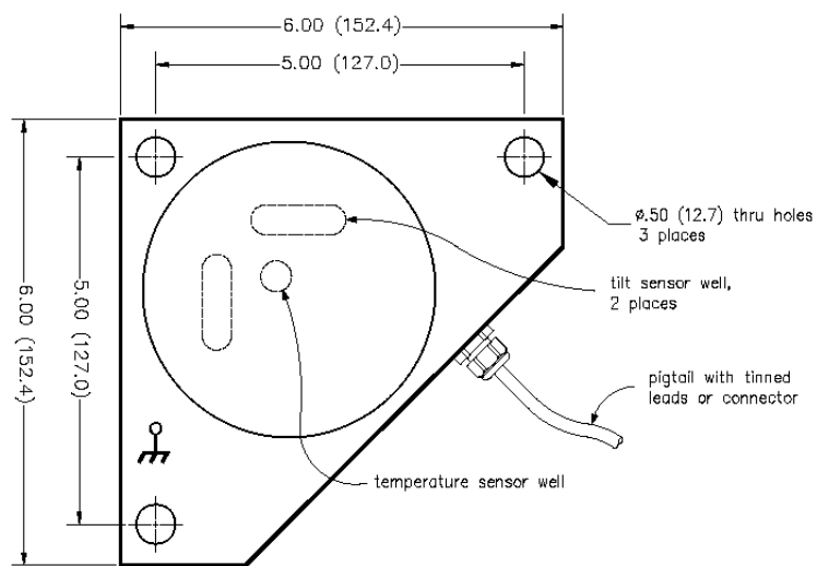
Top View Model D711 Digital Floor Mount Tiltmeter
