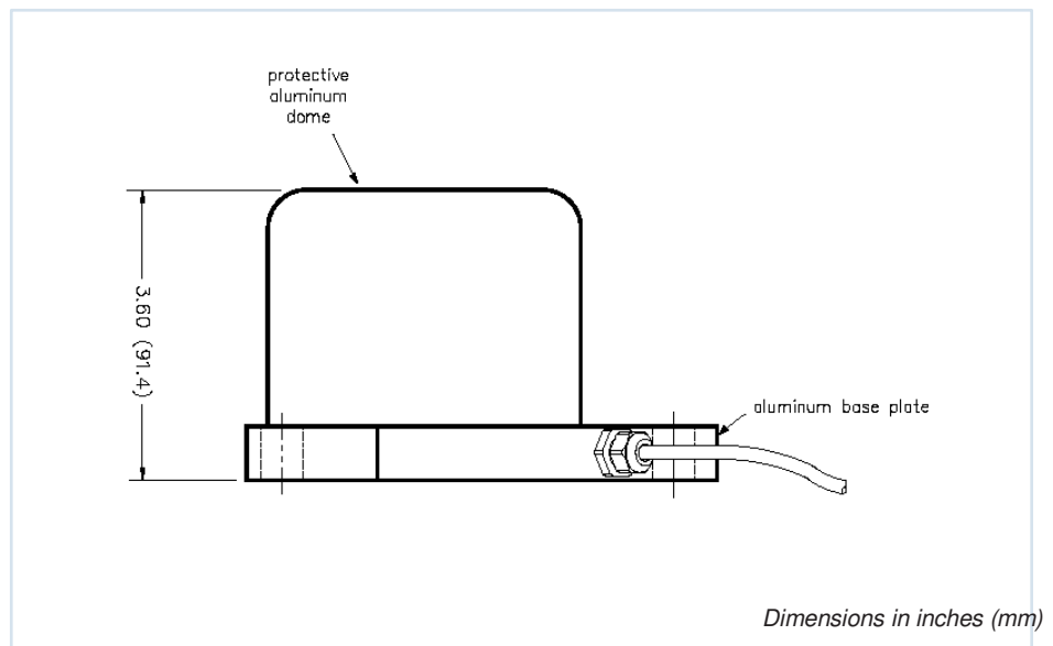
Side View Model D711 Digital Floor Mount Tiltmeter
