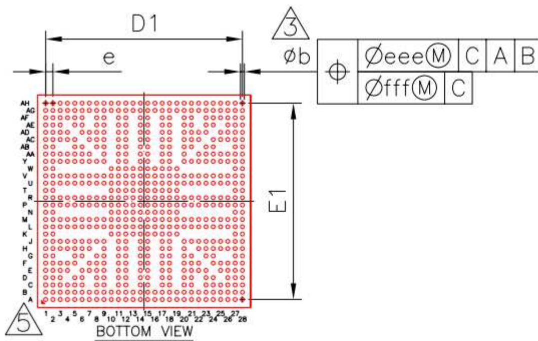
Fig. 2-3 RK3288 FCBGA636LD Package Bottom View
