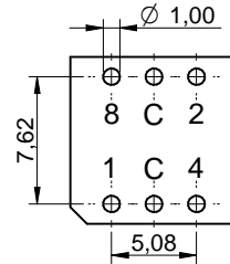
RECOMMENDED LAYOUT
