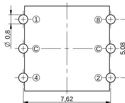
RECOMMENDED LAYOUT
