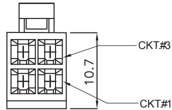
Dimensions for 4pins & 2pins connector
