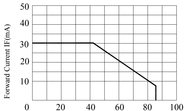
Fig.4 FORWARD CURRENT VS. DERATING CURVE
