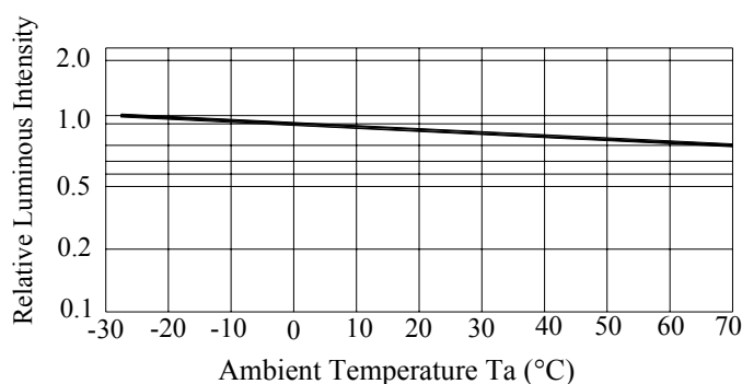
Fig.6 LUMINOUS INTENSITY VS. AMBIENT TEMPERATURE
