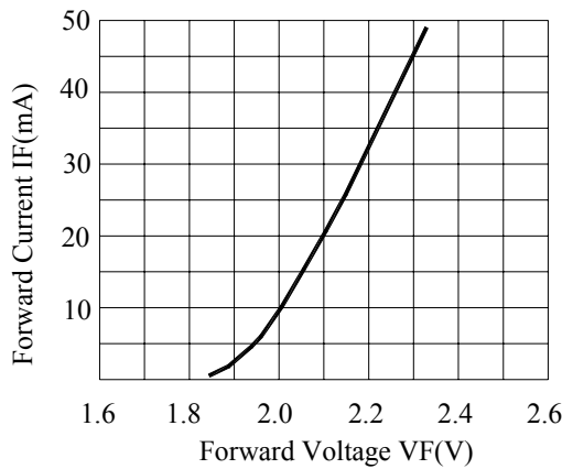
Fig.3 FORWARD CURRENT VS. FORWARD VOLTAGE PER CHIP
