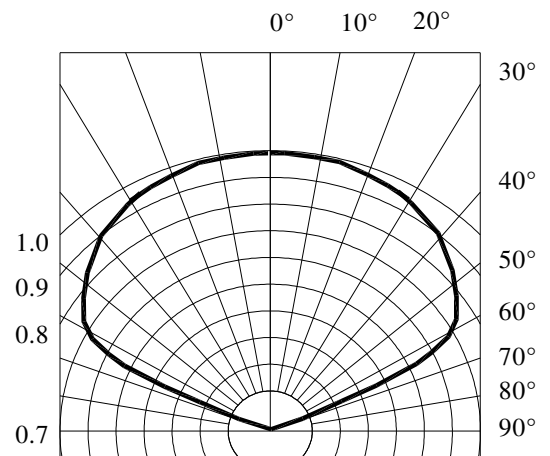
Radiation Diagram
