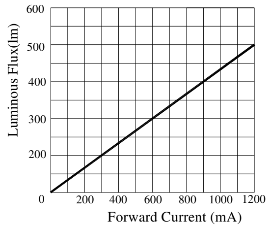
Forward Current VS. Luminous Flux
