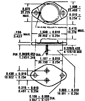
All dimensions in INCH / m.m. FIGURE 1
