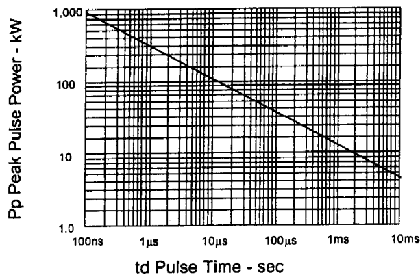
Fig. 2 - Peak Pulse Power vs. Pulse Time
