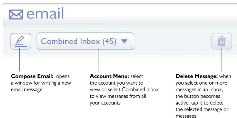
The Inbox selection menu and other email controls.
