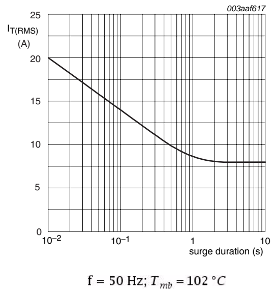
Fig 2. RMS on-state current as a function of surge duration; maximum value
