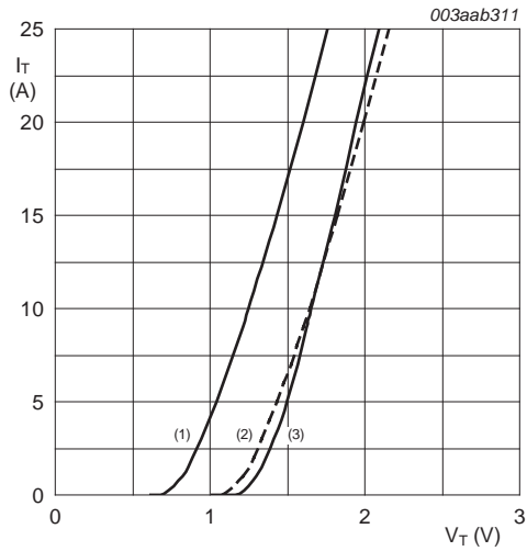
V_o = 1.26\text{ V} R_s = 0.0378\ \Omega (1) T_j = 125\text{ }^\circ\text{C} ; typical values (2) T_j = 125\text{ }^\circ\text{C} ; maximum values (3) T_j = 25\text{ }^\circ\text{C} ; maximum values
