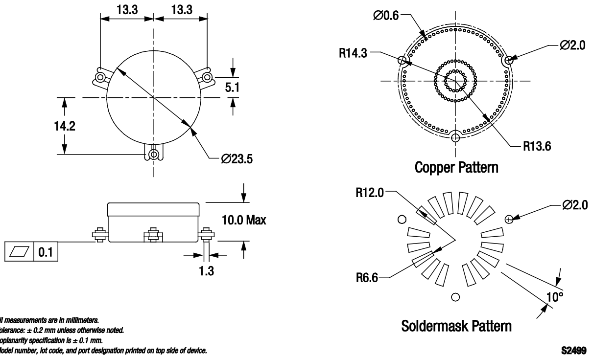
Figure 2. MAFR-000565-000001 Package Dimensions and PCB Footprint
