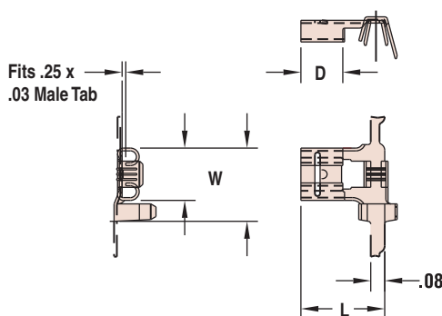
Flag Insulation Support Terminals
