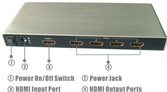
Figure 2. Rear Panel Layout
